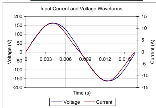
Input AC Current Waveform (ITHD = 7.75%, 50% Load)
