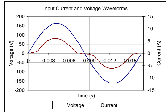
Input AC Current Waveform (ITHD = 27.27%, 50% Load)
