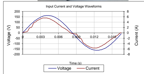
Input AC Current Waveform (ITHD = 13.78%, 50% Load)
