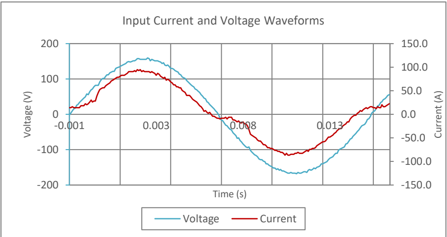
Input AC Current Waveform (ITHD = 16.08%, 50% Load)
