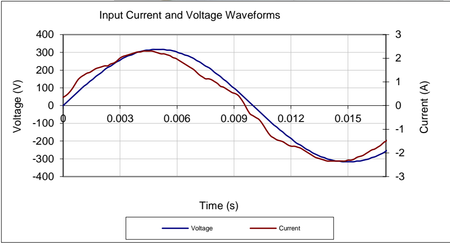
Input AC Current Waveform (ITHD = 9.16%, 50% Load)
