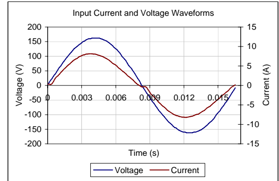
Input AC Current Waveform (ITHD = 12.48%, 50% Load)
