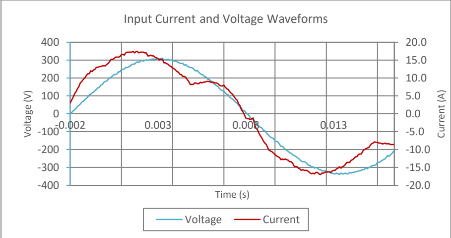
Input AC Current Waveform (ITHD = 17.04%, 50% Load)
