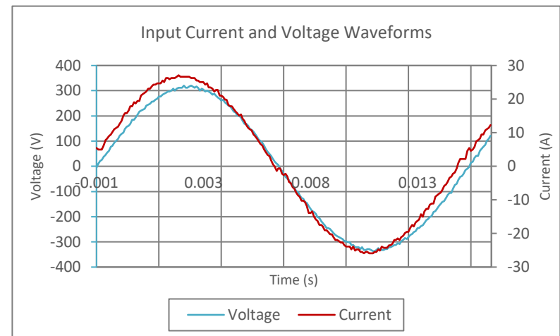
Input AC Current Waveform (ITHD = 2.29%, 50% Load)
