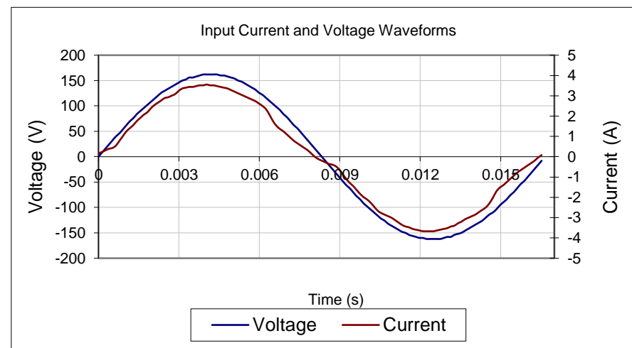
Input AC Current Waveform (ITHD = 8.12%, 50% Load)
