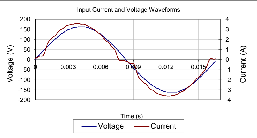
Input AC Current Waveform (ITHD = 9.3%, 50% Load)
